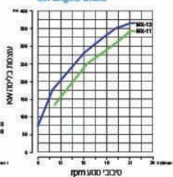
MX Engine Brake
